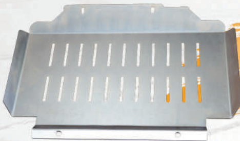
Part Number BP101-3 Ford Ranger PX3 - Third Plate Barcode 9319478660717 Fits at the end of the third (factory) bash plate for Transfer case protection RRP* $149.00
