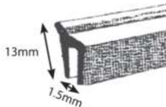
51-77976/100 Flare Edging
